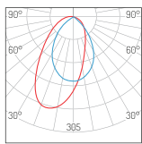
10W Wall Washer 2700K
