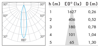
3W 15° 2700K
