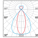
50W Rectangular+Batwing 3000K
