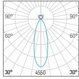
50W 30°+Batwing 3000K
